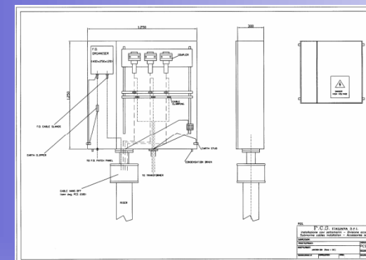
Vertical Accessible and Unaccessible Junction box
