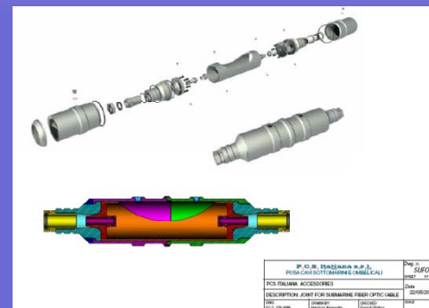
Submarine fibre optic joint
