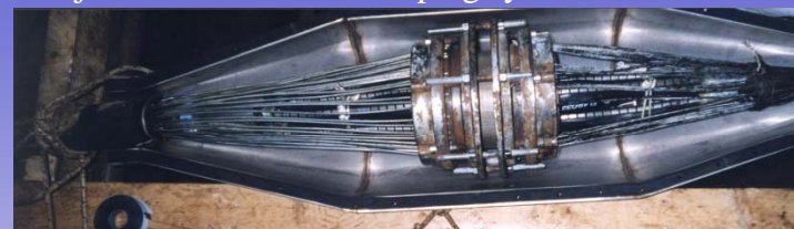
Submarine joints with armour clamping system
